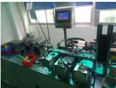
automatic assembly machines for male connectors
